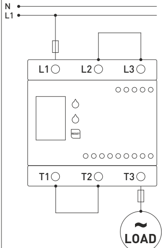
KON-TER-XX Connection Diagram (Mono-phase)
