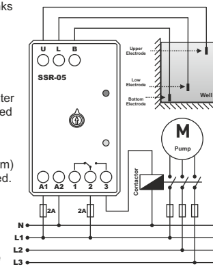
Connection diagrams for SSR-05
