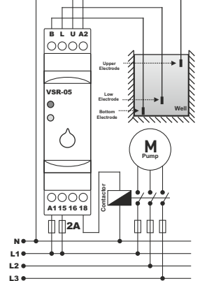
Connection diagrams for VSR-05
