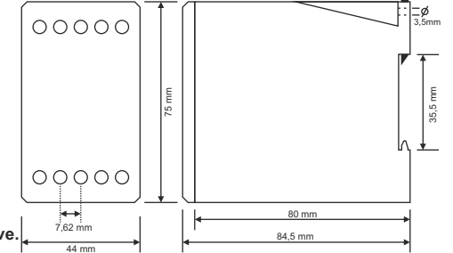
Dimensions for SSR-05
