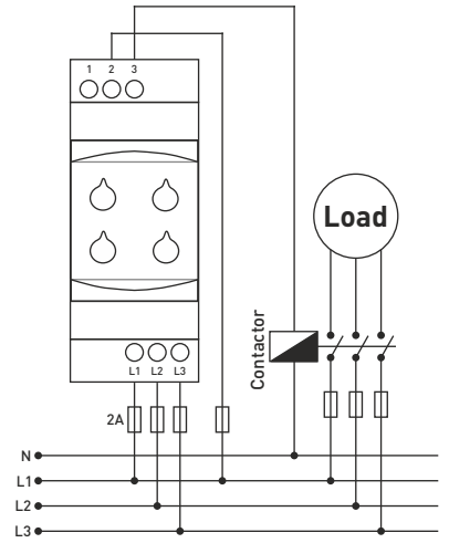
Connection Diagram for GKT-03/03F
