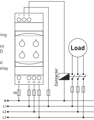
Connection Diagram for GKM-02/02F
